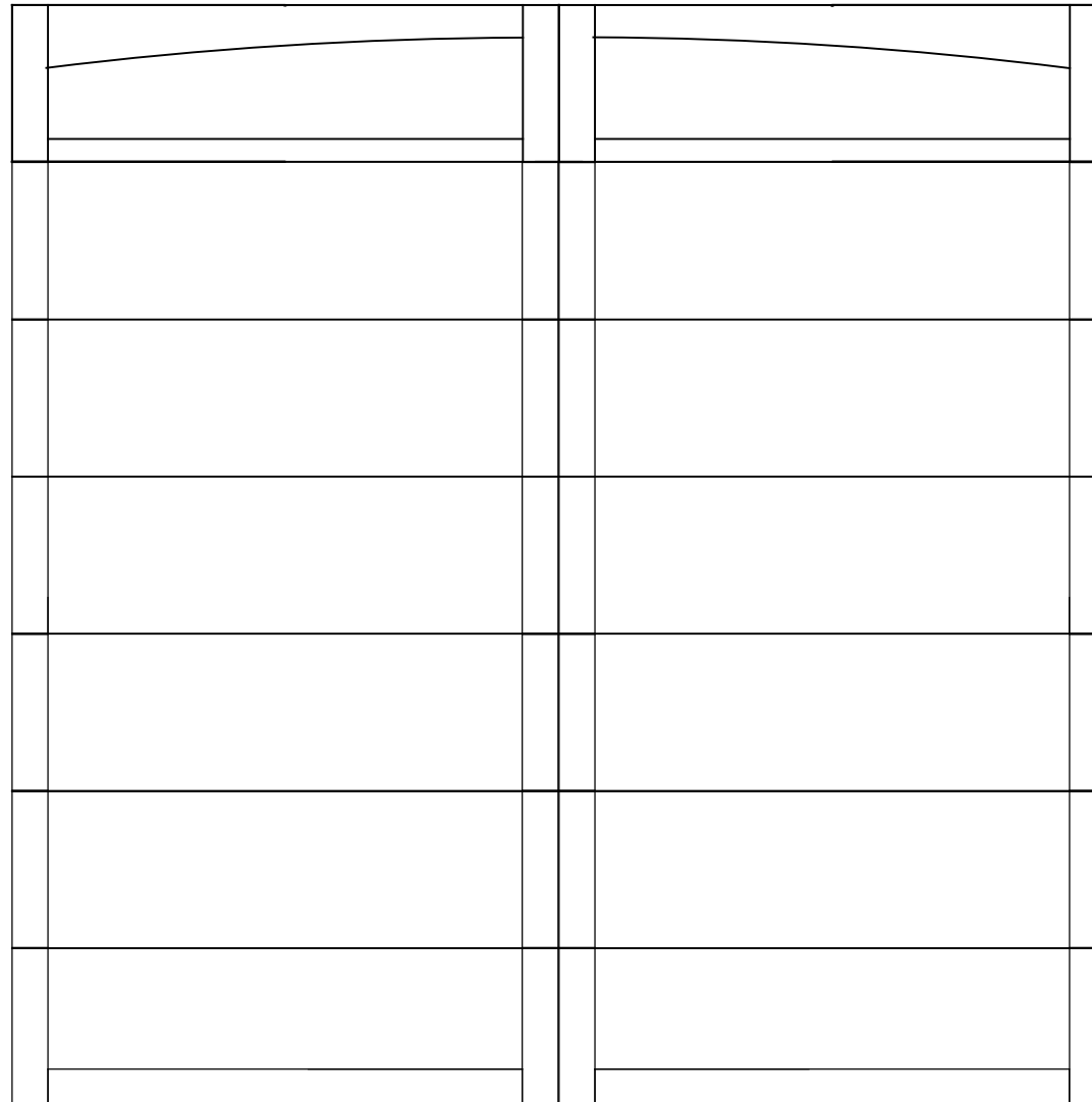
14x14 6600 ARLINGTON 7 SECTION/2 PANEL SOLID ARCH TOP SECTION SHOWN CONSISTS OF (7) 24.0" SECTIONS
