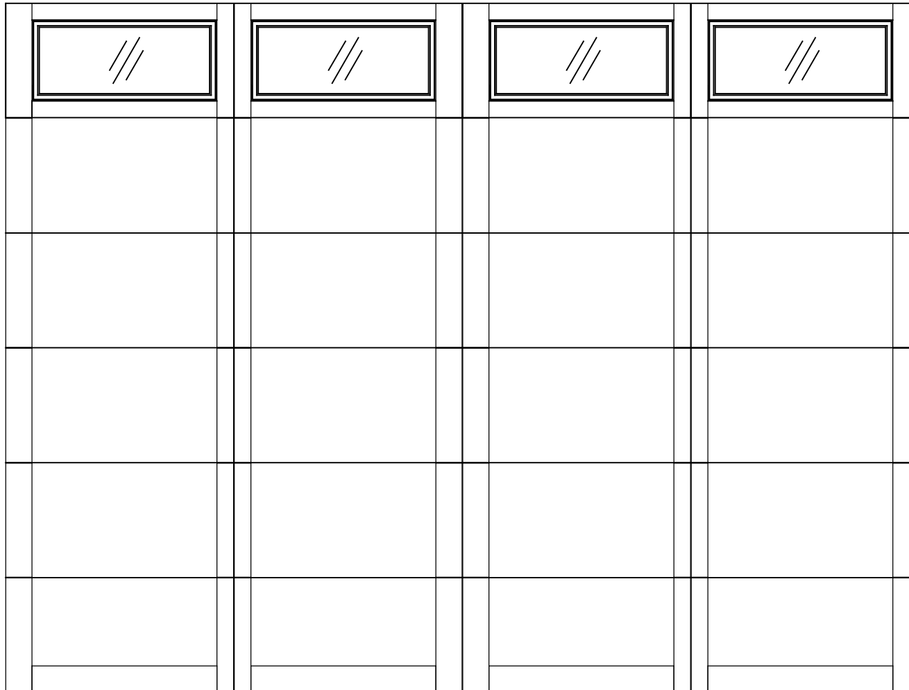
16x12 6600C ARLINGTON 6 SECTION/4 PANEL PLAIN GLAZE FRAMED TOP SECTION SHOWN CONSISTS OF (6) 24.0" SECTIONS
