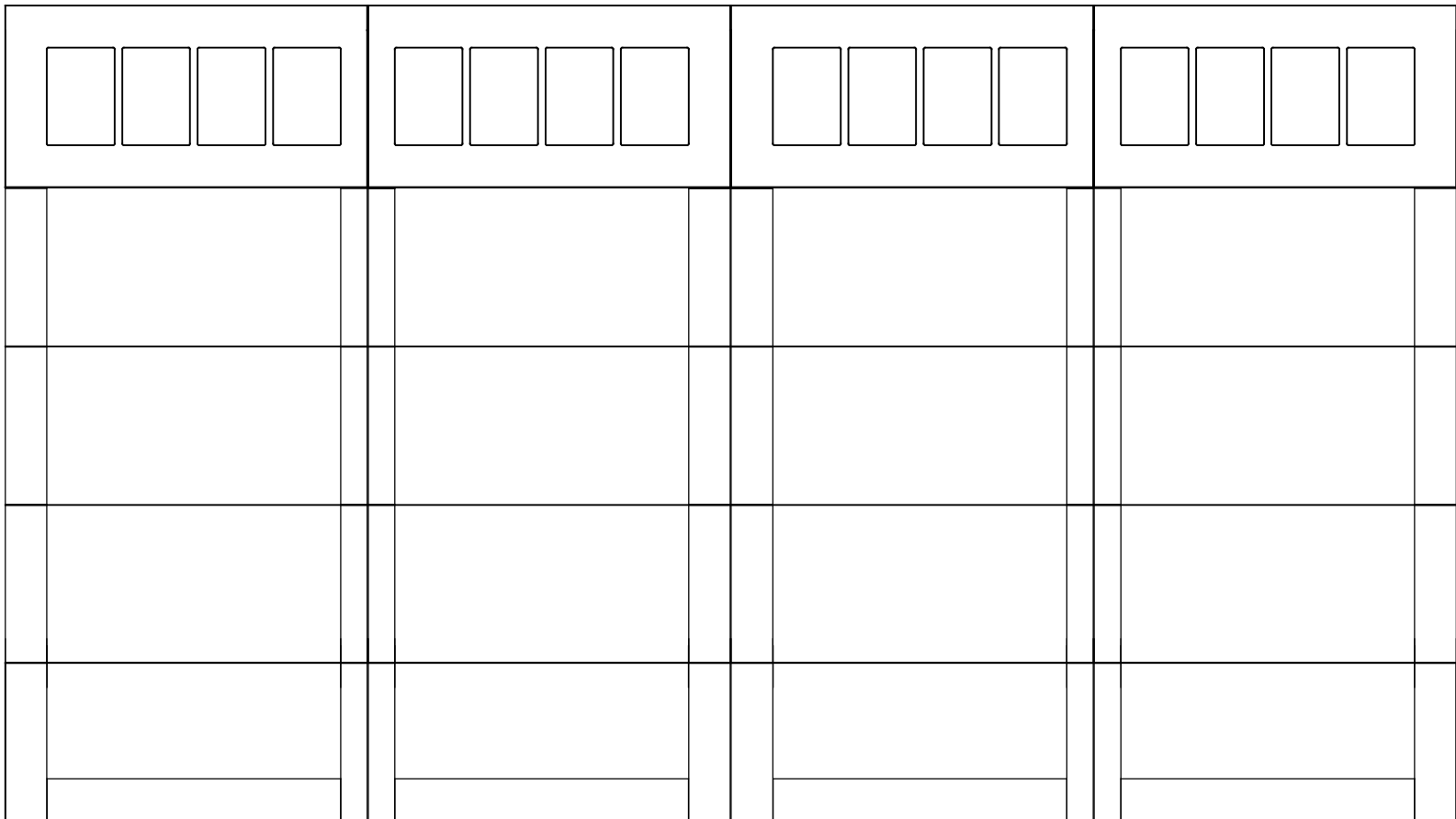
16x9 6600 ARLINGTON 5 SECTION/2 PANEL ROUTED STOCKBRIDGE TOP SECTION SHOWN CONSISTS OF (4) 20.8" & (1) 24" SECTIONS
