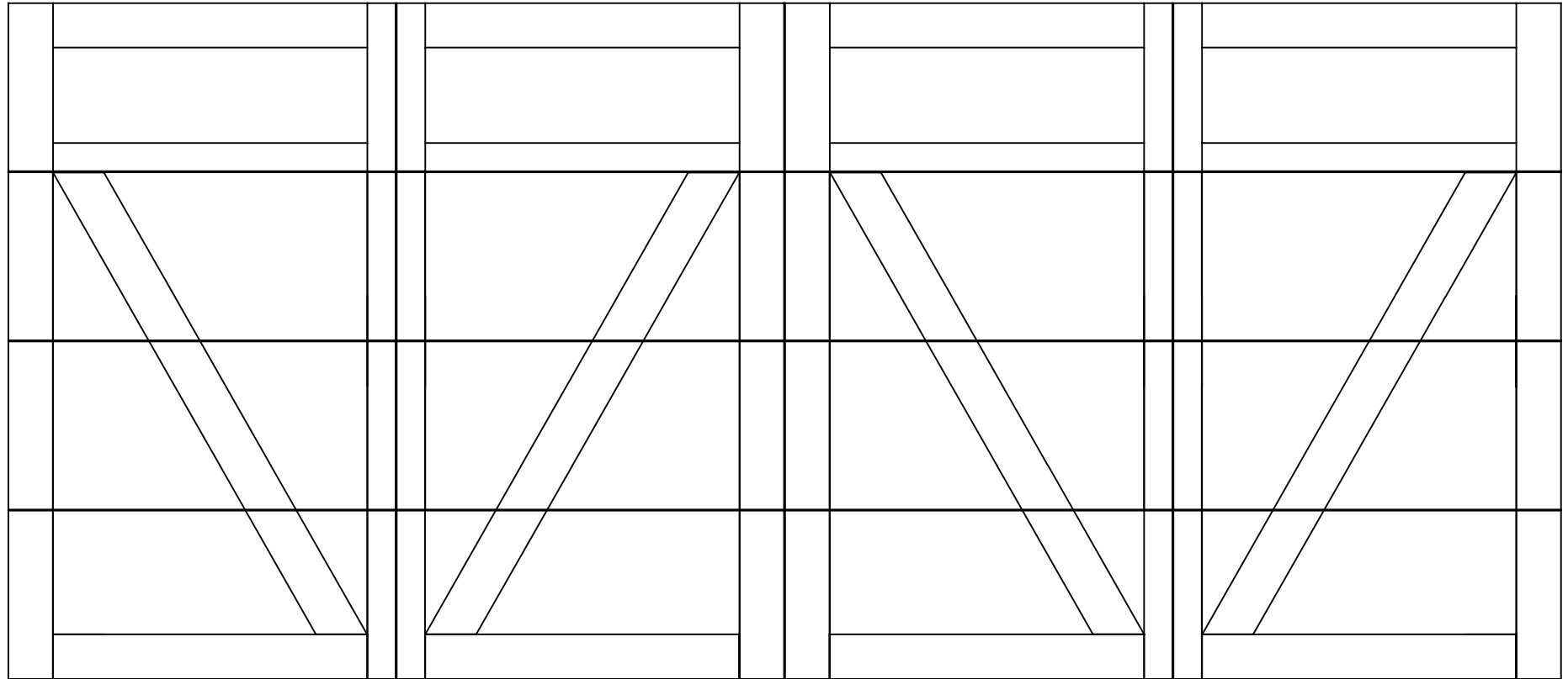
16x7 6600 Bellview 4 SECTION/4 PANEL SOLID SQUARE TOP SECTION SHOWN CONSISTS OF (4) 20.8" SECTIONS
