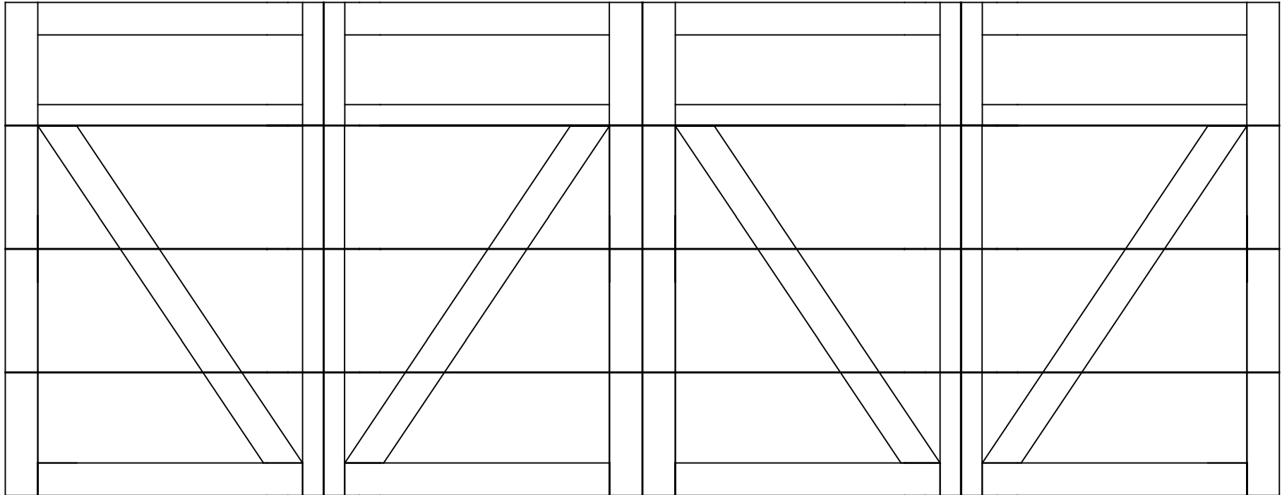
18x7 6600 Bellview 4 SECTION/4 PANEL SOLID SQUARE TOP SECTION SHOWN CONSISTS OF (4) 20.8" SECTIONS
