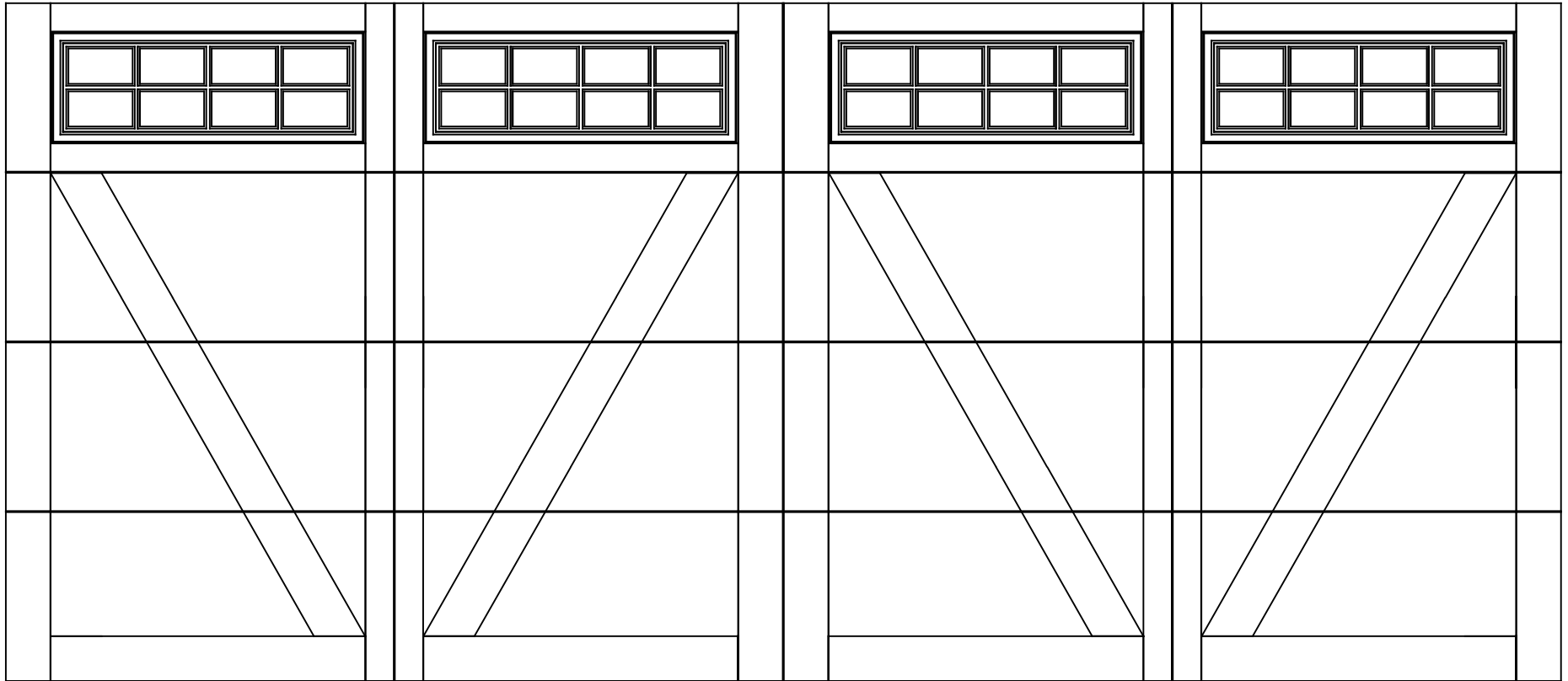
16x7 6600 BELLVIEW 4 SECTION/4 PANEL FRAMED STOCKTON TOP SECTION SHOWN CONSISTS OF (4) 20.8" SECTIONS
