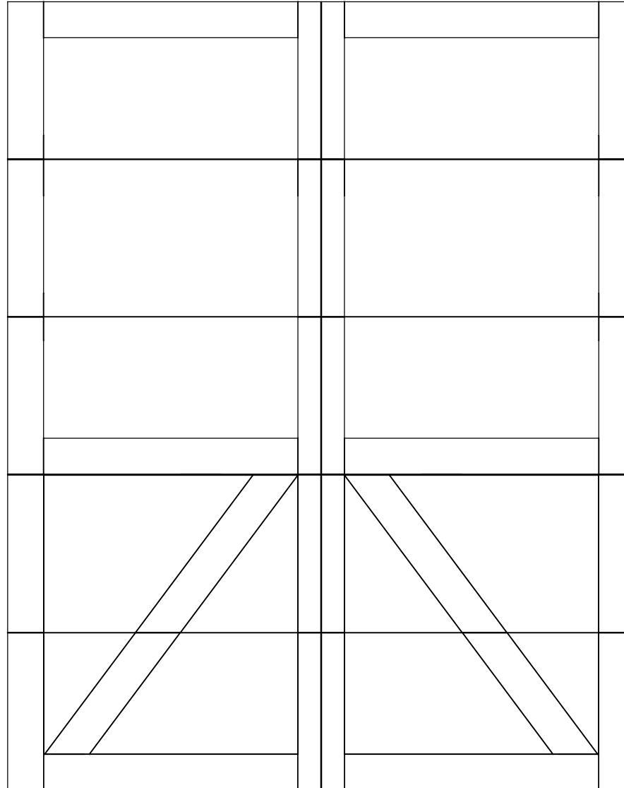
8 X 10 6600 KINGSTON 5 SECTION/2 PANEL SOLID SQUARE TOP SECTION SHOWN CONSISTS OF (5) 24.0" SECTIONS
