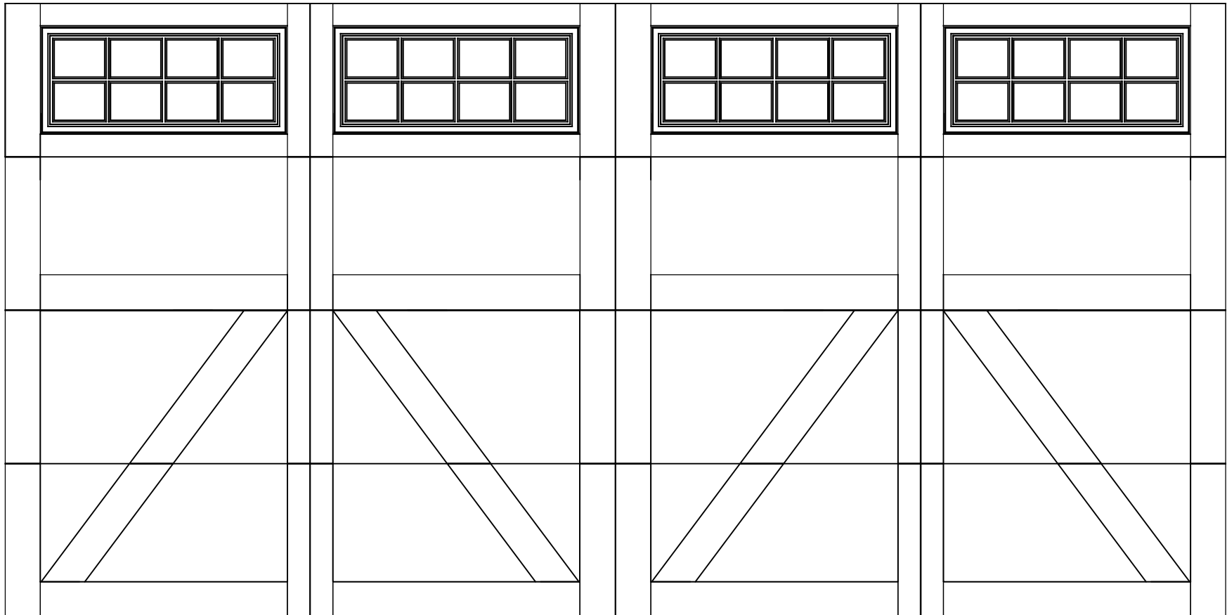
16 X 8 6600 KINGSTON 4 SECTION/4 PANEL FRAMED STOCKTON TOP SECTION SHOWN CONSISTS OF (4) 24.0" SECTIONS
