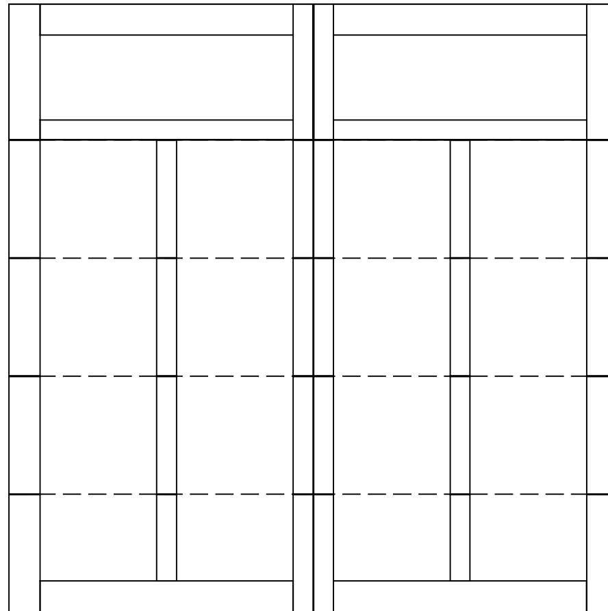
9'x9' 6600 SOMERSET 5 SECTION/2 PANEL SOLID SQUARE TOP SECTION SHOWN CONSISTS OF (4) 20.8" SECTIONS AND (1) 24.0" SECTIONS
