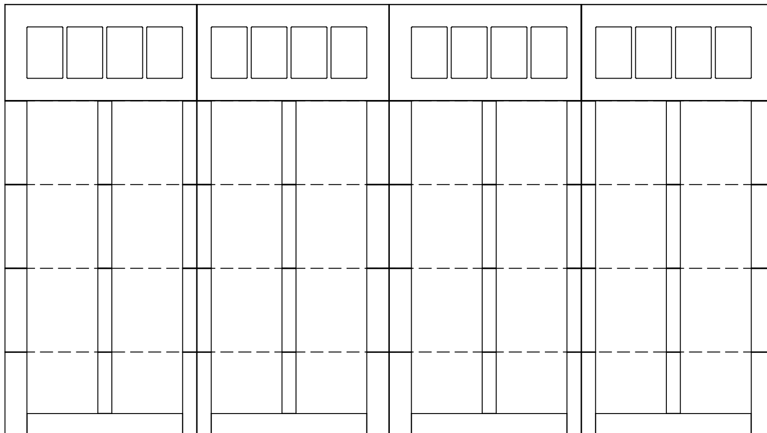
16'x9' 6600 SOMERSET 5 SECTION/4 PANEL ROUTED STOCKBRIDGE TOP SECTION SHOWN CONSISTS OF (4) 20.8" SECTIONS AND (1) 24.0" SECTIONS
