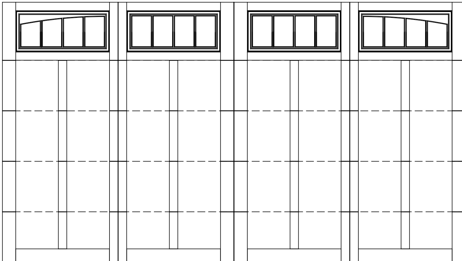
16'x9' 6600 SOMERSET 5 SECTION/4 PANEL FRAMED SINGLE WYNDBRIDGE TOP SECTION SHOWN CONSISTS OF (4) 20.8" SECTIONS AND (1) 24.0" SECTIONS
