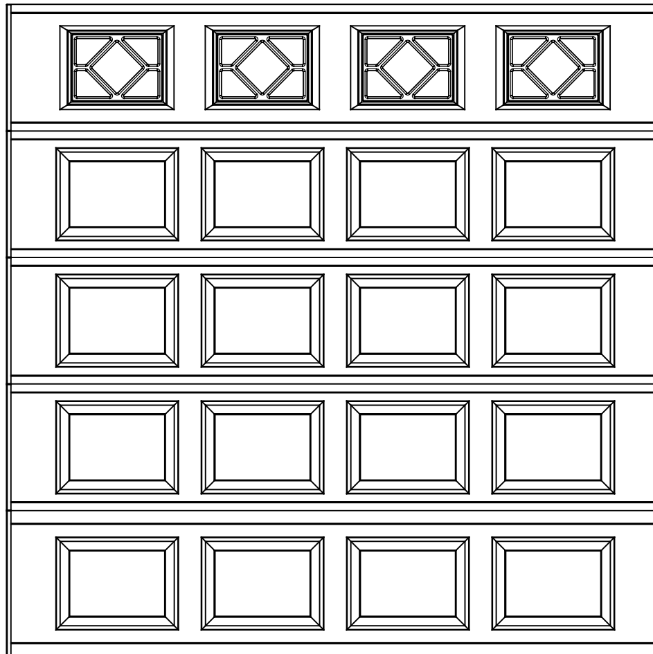
9'0" X 9'0" 8300/8500 CRP DESIGN 5 SECTION/4 PANEL WATERTON I TOP SECTION SHOWN (4) 20.8" & (1) 24" SECTIONS
