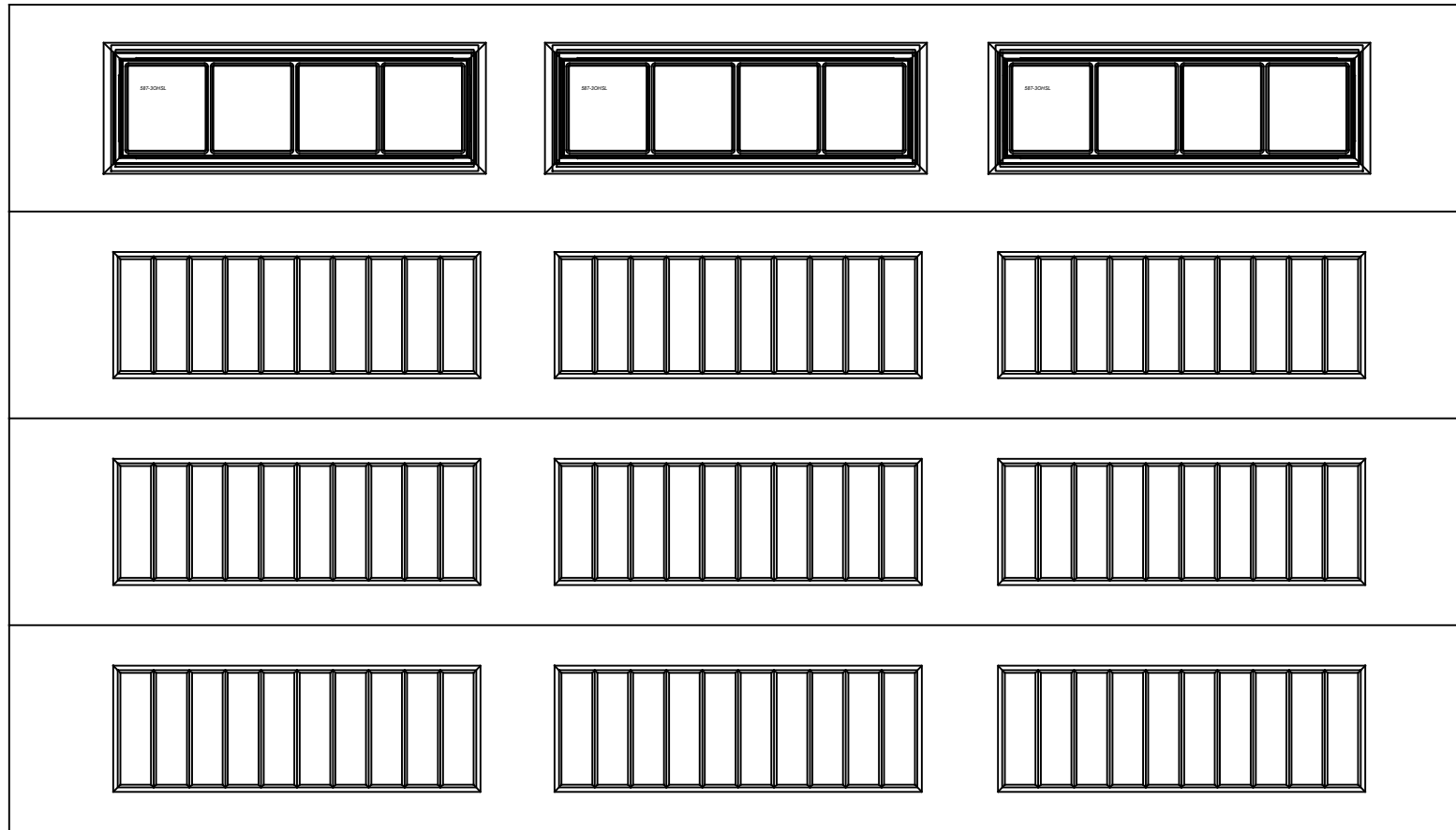
14 X 8 9605 SONOMA RANCH 4 SECTIONS/3 PANELS STOCKBRIDGE IV 4 LITE TOP SECTION SHOWN CONSISTS OF (4) 23.8" SECTIONS
