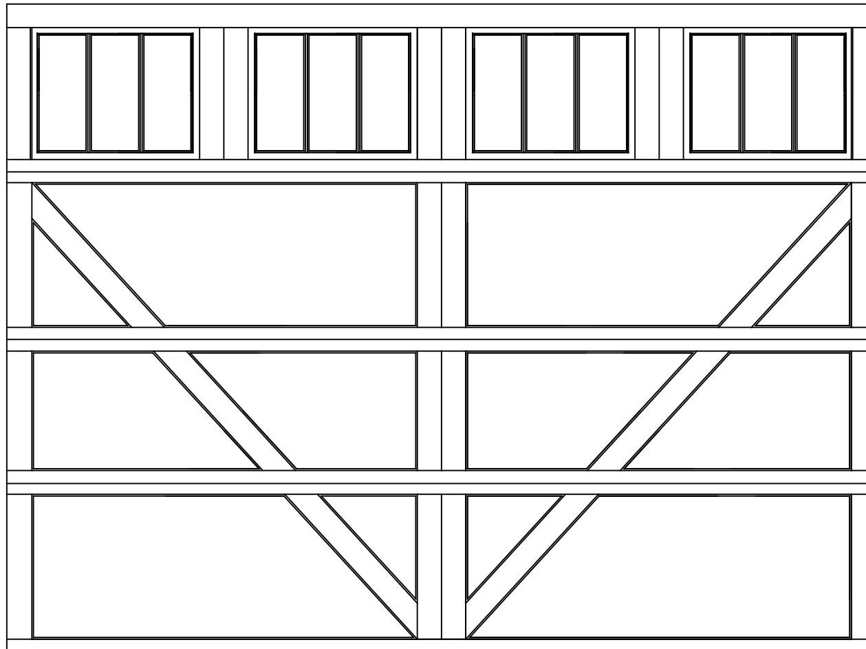
12' X 9' 9700 BELLVIEW DESIGN 4 SECTION/2 PANEL 12 LITE SQUARE TOP SECTION SHOWN (1) 23.8" & (3) 27.73" SECTIONS
