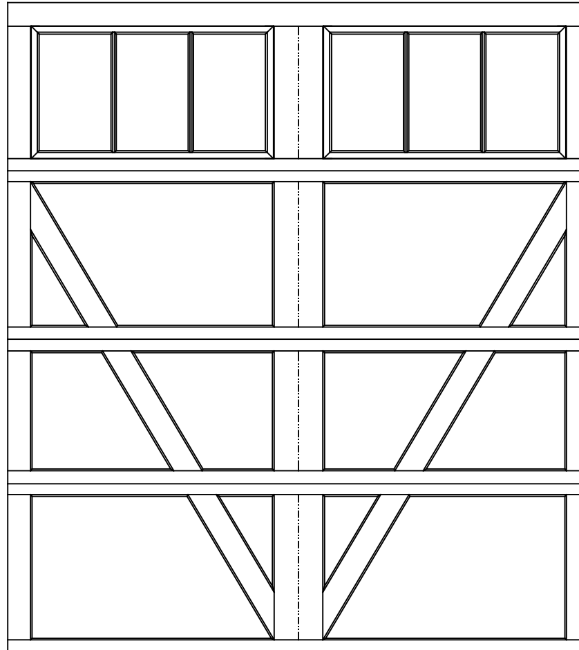
8'0" X 9'0" 9700 BELLVIEW DESIGN 4 SECTION/2 PANEL 6 LITE TOP SECTION SHOWN (1) 23.8" & (3) 27.73" SECTIONS
