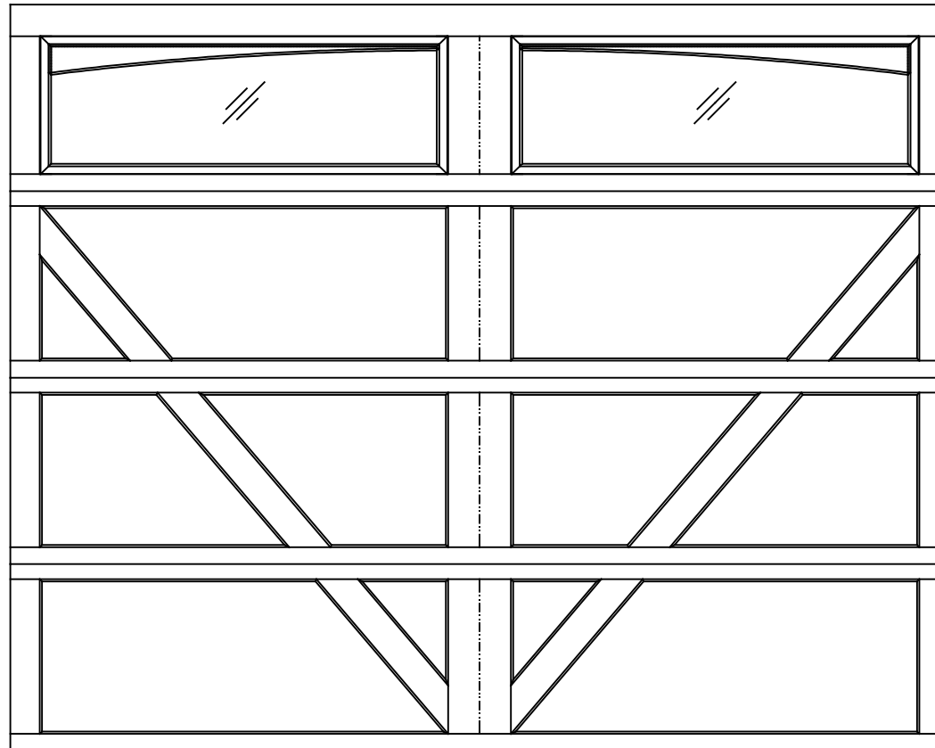
10'0" X 8'0" 9700 BELLVIEW DESIGN 4 SECTION/2 PANEL PLAIN ARCHED TOP SECTION SHOWN (4) 23.8" SECTIONS
