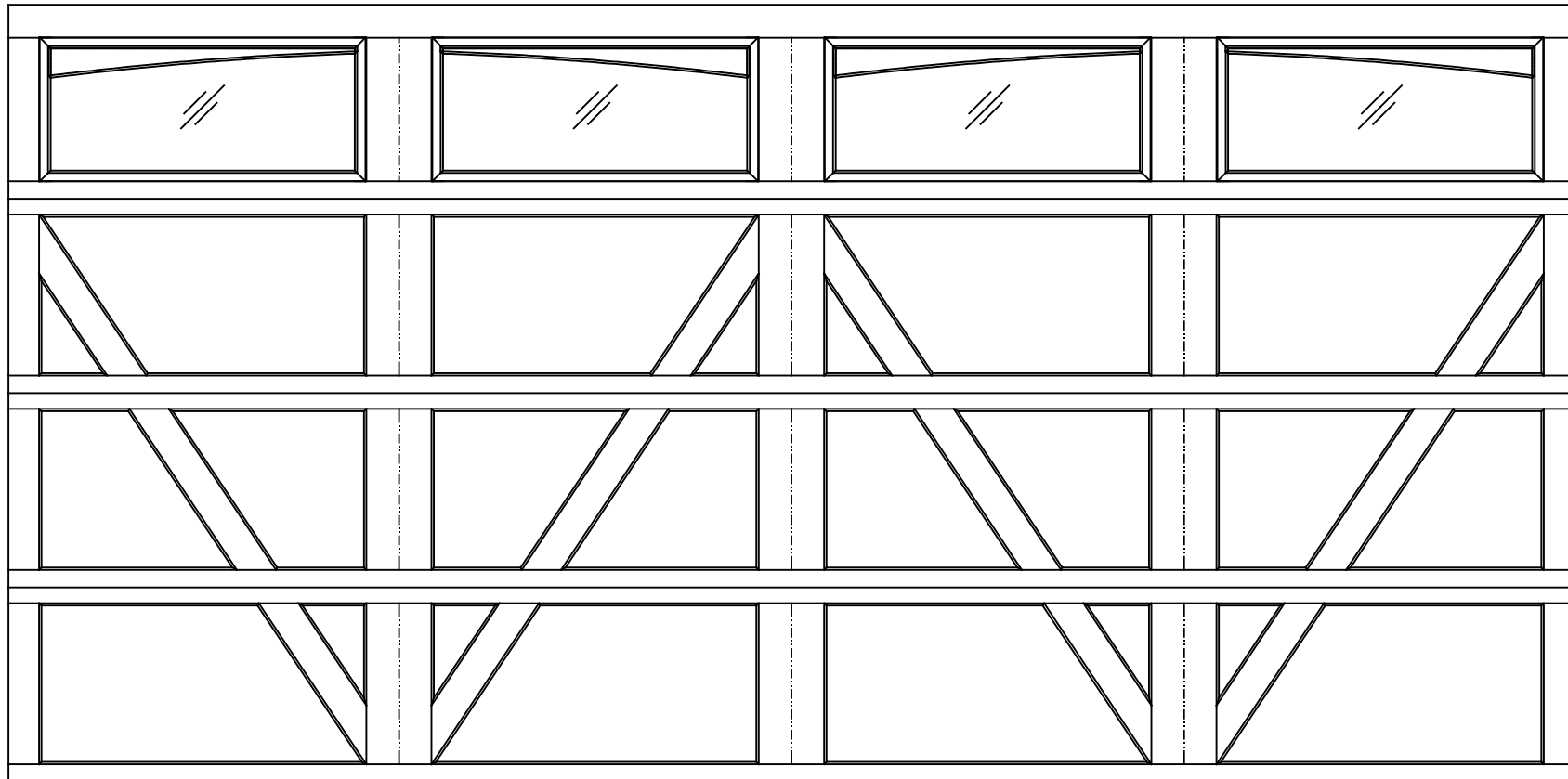
16'0" X 8'0" 9700 BELLVIEW DESIGN 4 SECTION/4 PANEL DOUBLE PLAIN ARCHED TOP SECTION SHOWN (4) 23.8" SECTIONS
