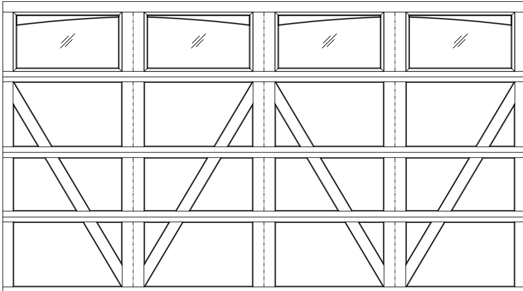
16'0" X 9'0" 9700 BELLVIEW DESIGN 4 SECTION/2 PANEL DOUBLE PLAIN ARCHED TOP SECTION SHOWN (1) 23.8" & (3) 27.73" SECTIONS
