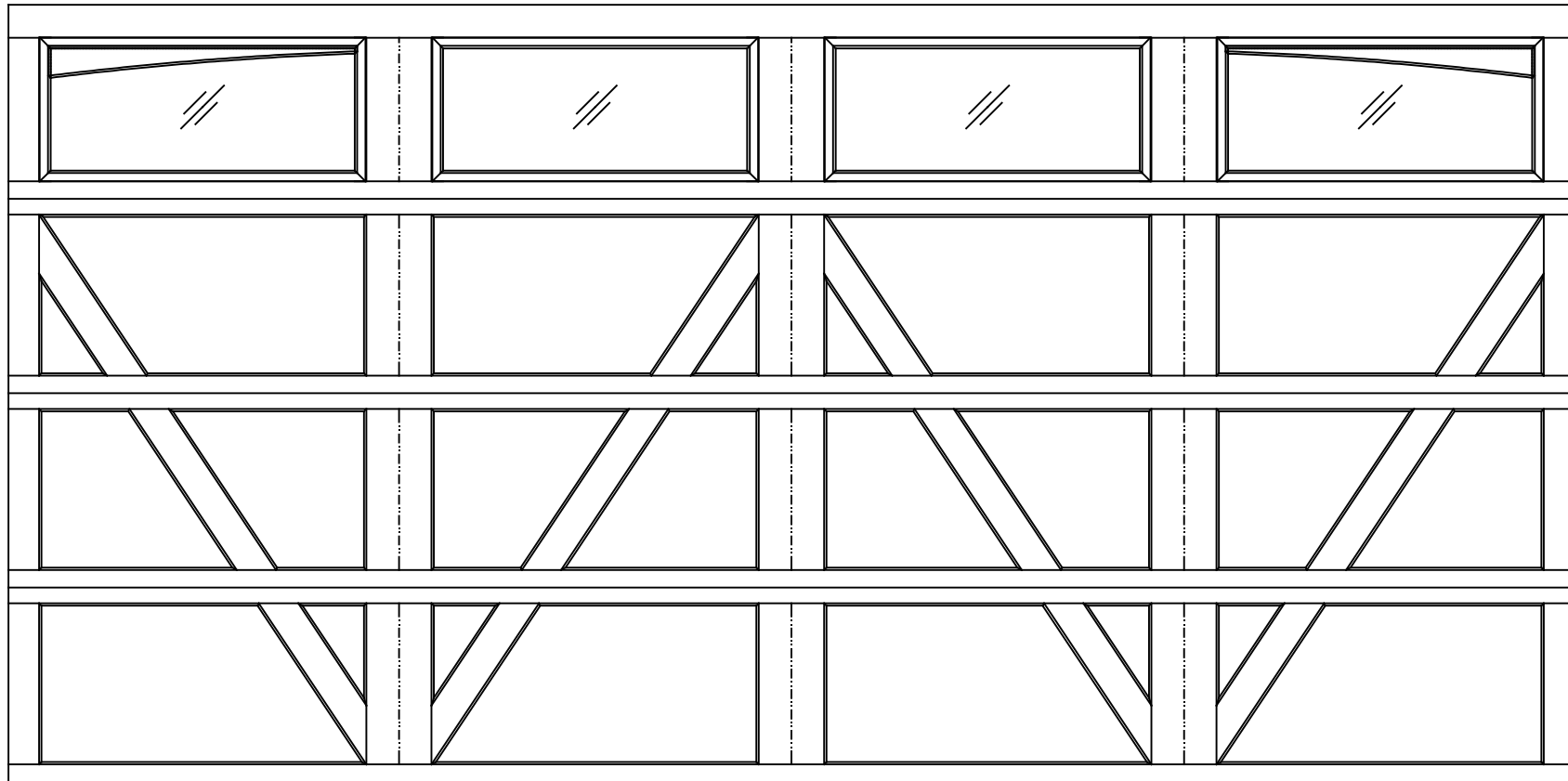
16'0" X 8'0" 9700 BELLVIEW DESIGN 4 SECTION/4 PANEL SINGLE PLAIN ARCHED TOP SECTION SHOWN (4) 23.8" SECTIONS
