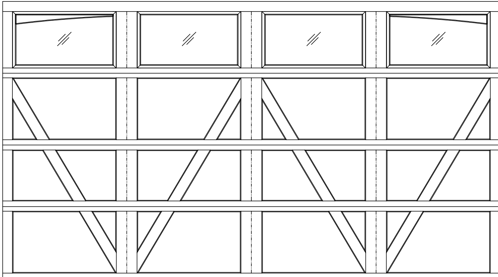
16'0" X 9'0" 9700 BELLVIEW DESIGN 4 SECTION/2 PANEL SINGLE PLAIN ARCHED TOP SECTION SHOWN (1) 23.8" & (3) 27.73" SECTIONS
