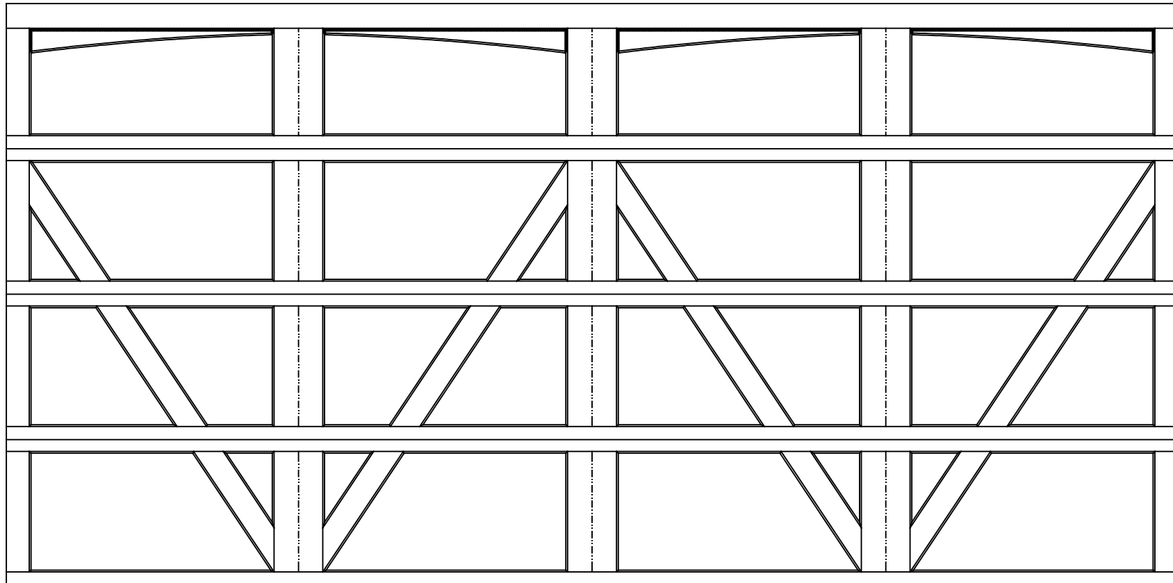
16'0" X 8'0" 9700 BELLVIEW DESIGN 4 SECTION/4 PANEL DOUBLE SOLID ARCHED TOP SECTION SHOWN (4) 23.8" SECTIONS
