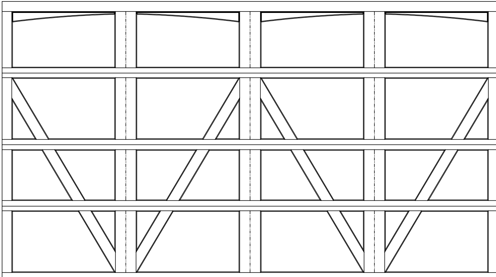
16'0" X 9'0" 9700 BELLVIEW DESIGN 4 SECTION/2 PANEL DOUBLE SOLID ARCHED TOP SECTION SHOWN (1) 23.8" & (3) 27.73" SECTIONS
