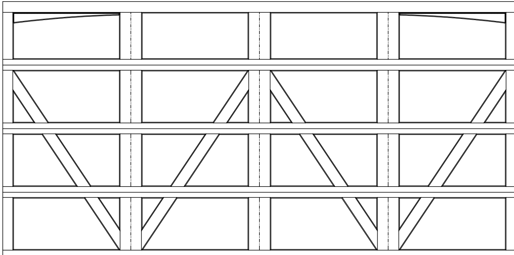
16'0" X 8'0" 9700 BELLVIEW DESIGN 4 SECTION/4 PANEL SINGLE SOLID ARCHED TOP SECTION SHOWN (4) 23.8" SECTIONS
