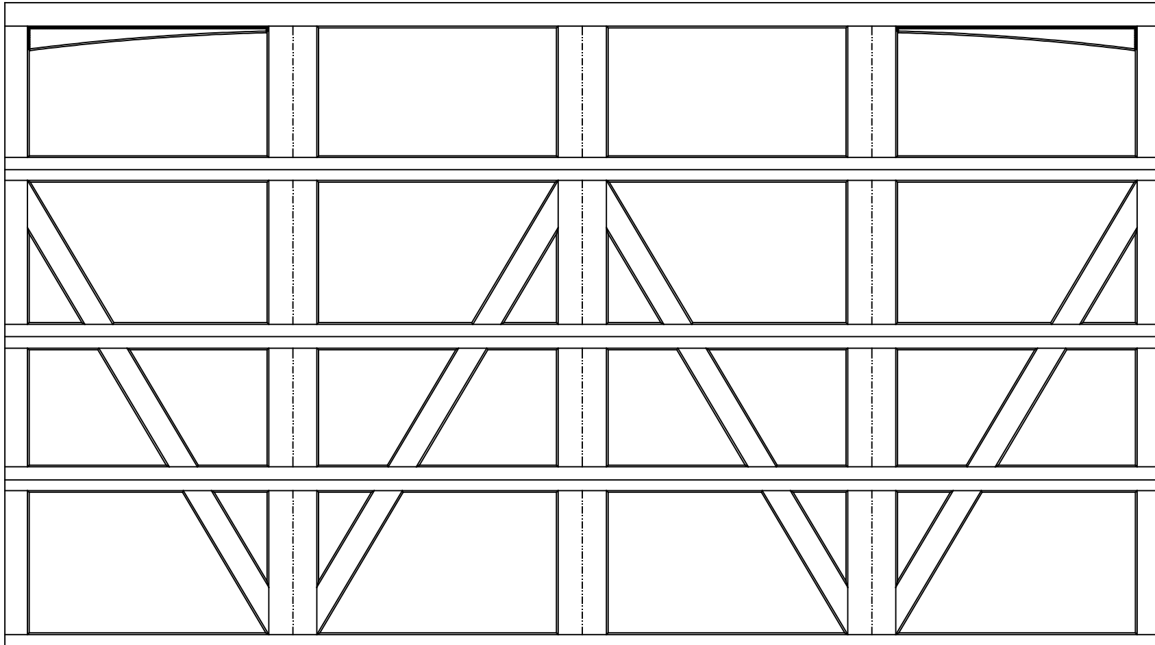
16'0" X 9'0" 9700 BELLVIEW DESIGN 4 SECTION/2 PANEL SINGLE SOLID ARCHED TOP SECTION SHOWN (1) 23.8" & (3) 27.73" SECTIONS
