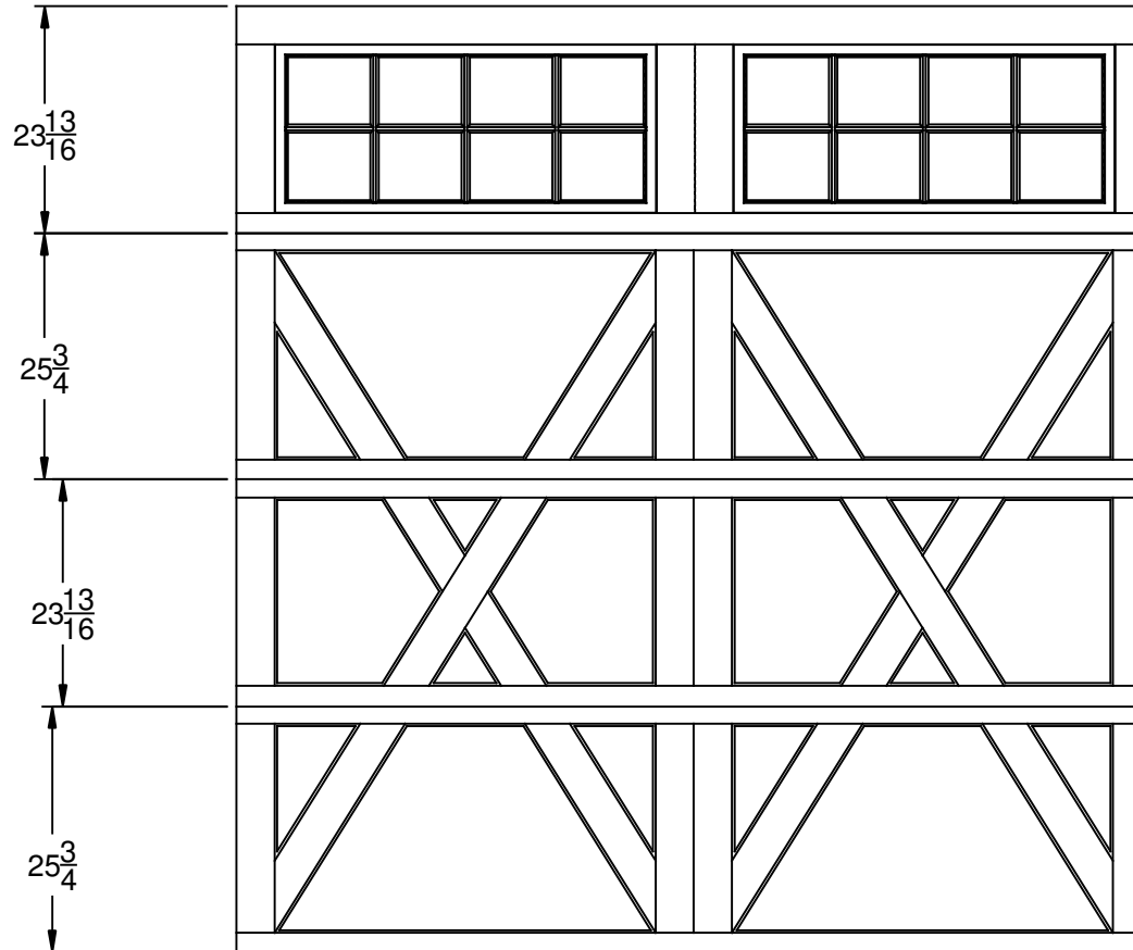
8'x8'6" 9700 LEXINGTON DESIGN 4 SECTION/2 PANEL 16 LITE SQUARE TOP SECTION SHOWN CONSISTS OF (2) 23.8" & (2) 25.73" SECTIONS
