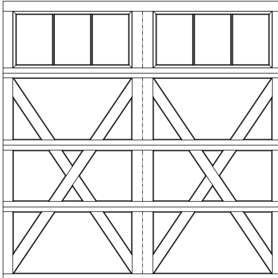
9'0" X 9'0" 9700 LEXINGTON DESIGN 4 SECTION/2 PANEL 6 LITE TOP SECTION SHOWN (1) 23.8" & (3) 27.73" SECTIONS
