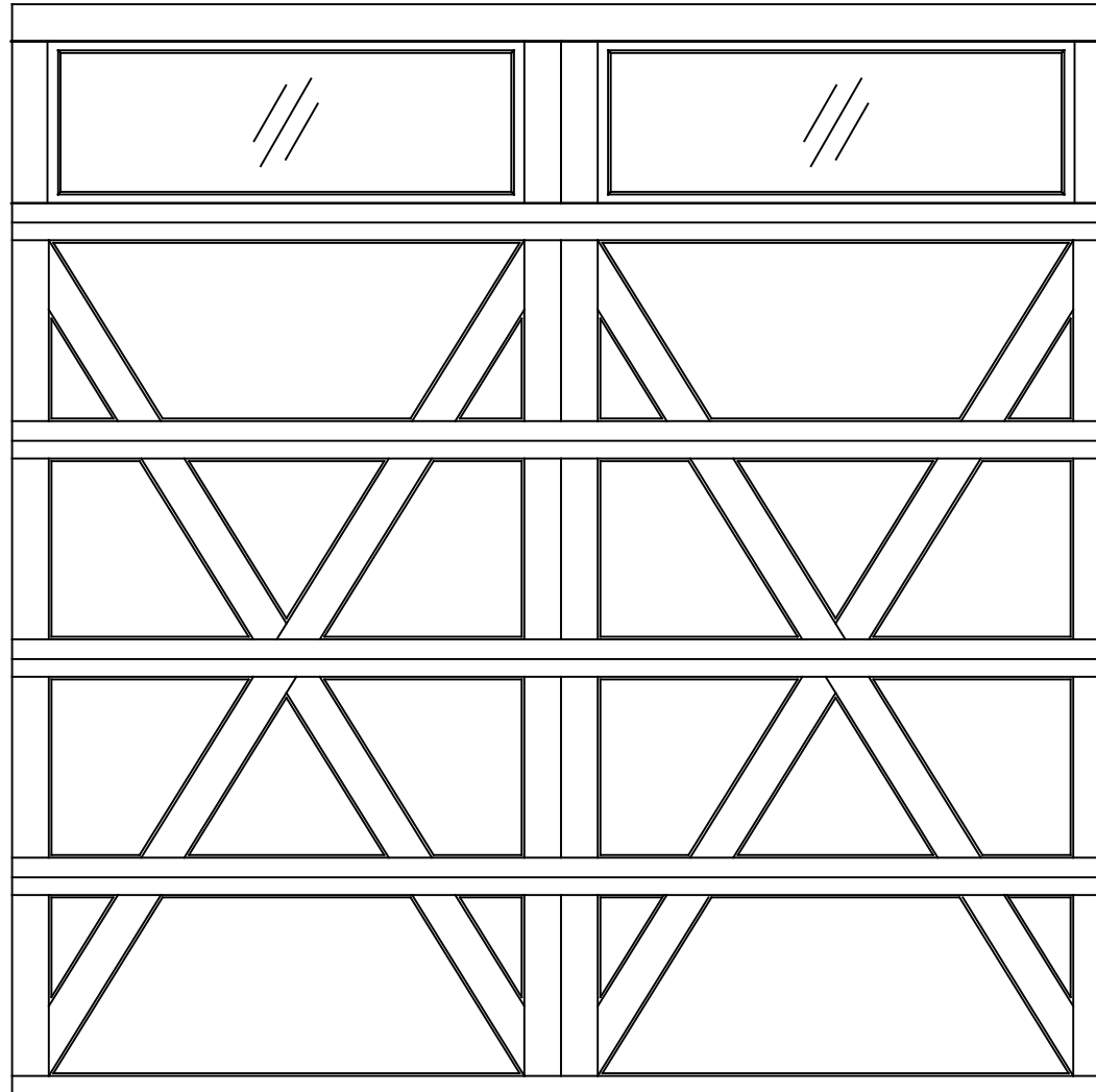
10 x 10 9700 LEXINGTON DESIGN 5 SECTION/2 PANEL PLAIN GLAZED SQUARE TOP SECTION SHOWN CONSISTS OF (5) 23.8" SECTIONS
