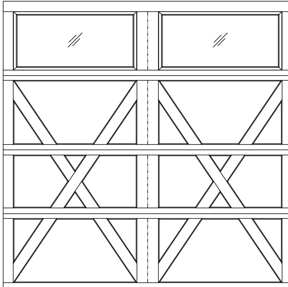
9'0" X 9'0" 9700 LEXINGTON DESIGN 4 SECTION/2 PANEL PLAIN TOP SECTION SHOWN (1) 23.8" & (3) 27.73" SECTIONS
