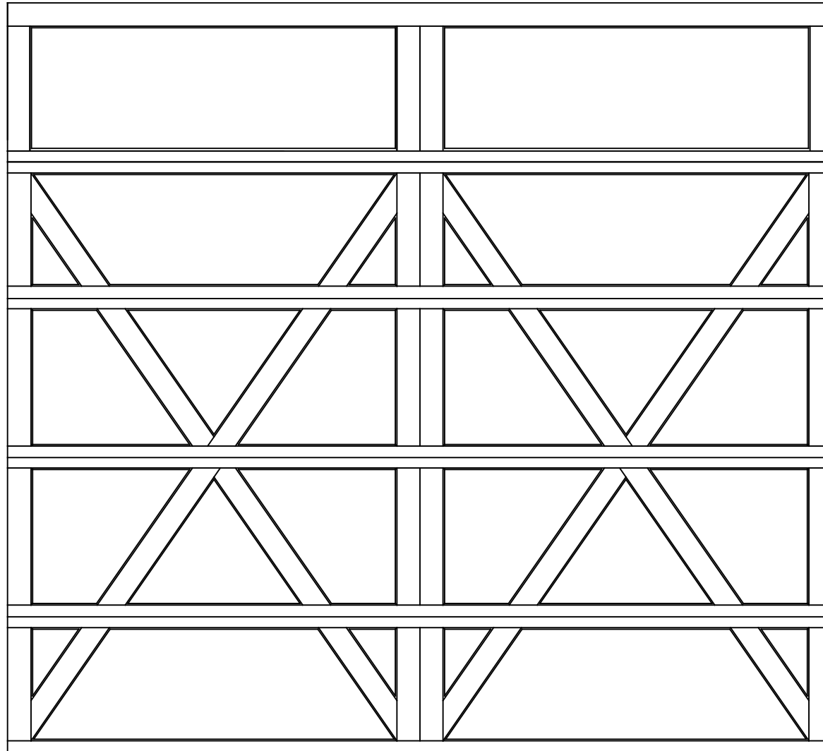
12x11 9700 LEXINGTON DESIGN 5 SECTION/2 PANEL SOLID SQUARE TOP SECTION SHOWN CONSISTS OF (2) 23.8" & (3) 27.73" SECTIONS
