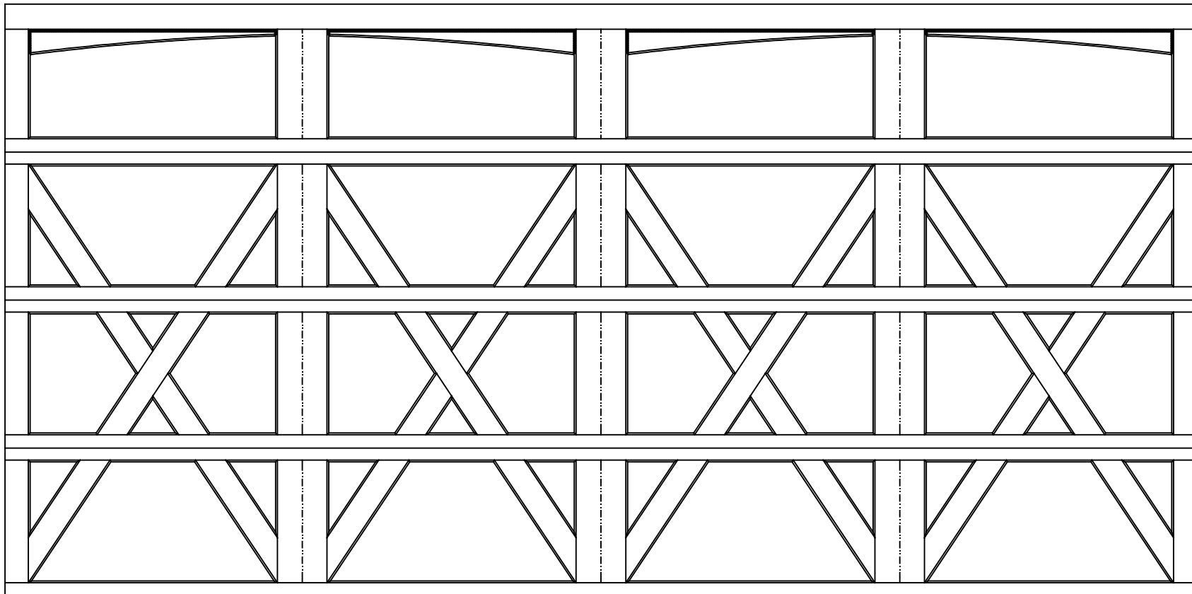
16'0" X 8'0" 9700 LEXINGTON DESIGN 4 SECTION/4 PANEL DOUBLE SOLID ARCHED TOP SECTION SHOWN (4) 23.8" SECTIONS
