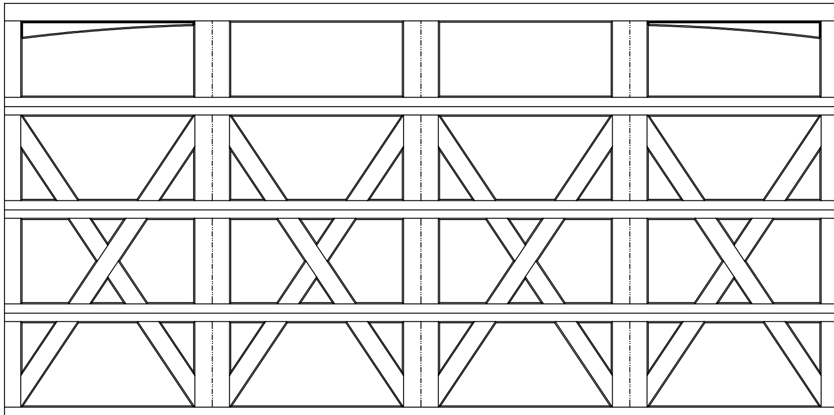
16'0" X 8'0" 9700 LEXINGTON DESIGN 4 SECTION/4 PANEL SINGLE SOLID ARCHED TOP SECTION SHOWN (4) 23.8" SECTIONS
