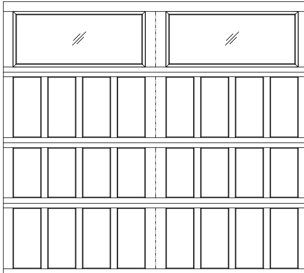
10'0" X 9'0" 9700 OAK PARK DESIGN 4 SECTION/2 PANEL PLAIN TOP SECTION SHOWN (1) 23.8" & (3) 27.73" SECTIONS
