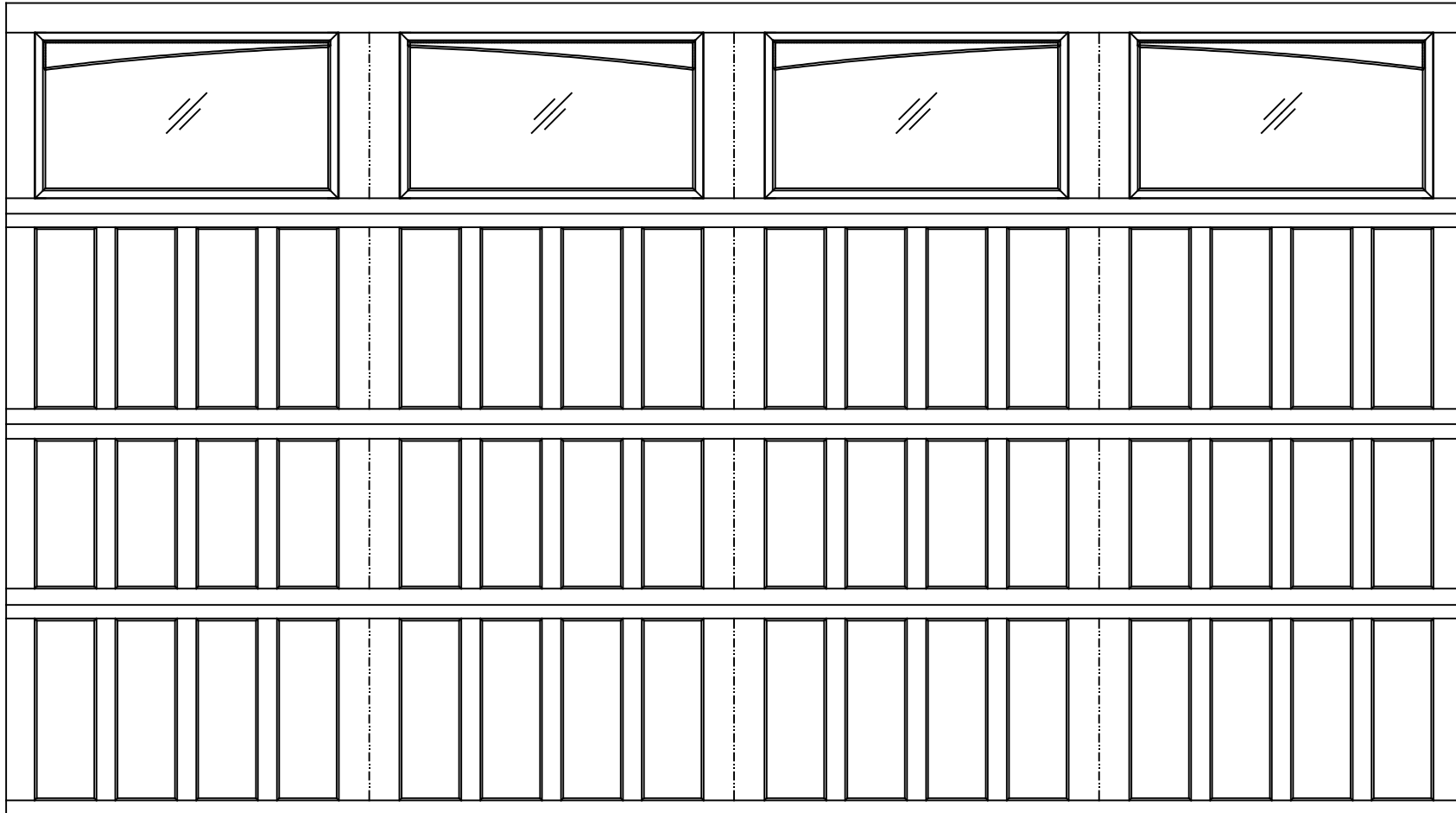
16'0" X 9'0" 9700 OAK PARK DESIGN 4 SECTION/4 PANEL DOUBLE PLAIN ARCHED TOP SECTION SHOWN (1) 23.8" & (3) 27.73" SECTIONS
