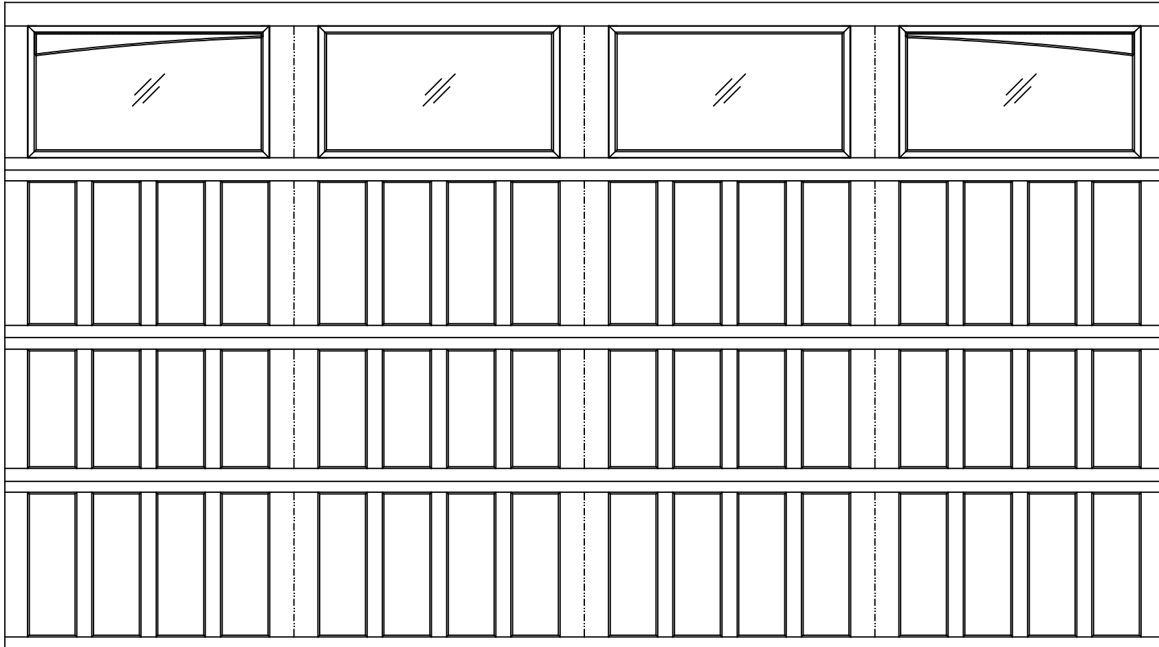
16'0" X 9'0" 9700 OAK PARK DESIGN 4 SECTION/4 PANEL SINGLE PLAIN ARCHED TOP SECTION SHOWN (1) 23.8" & (3) 27.73" SECTIONS
