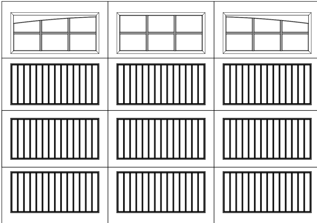
12' x 8'5" 9800 SONOMA 4 SECTION/3 PANEL 18 LITE ARCH TOP SECTION SHOWN CONSISTS OF (3) 25.73" & (1) 23.8" SECTIONS
