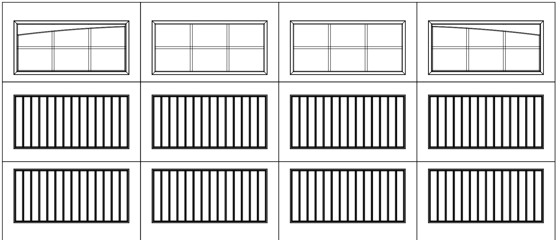
16x7 9800 SONOMA 3 SECTION/4 PANEL 24 LITE SINGLE ARCH TOP SECTION SHOWN CONSISTS OF (3) 27.73" SECTIONS
