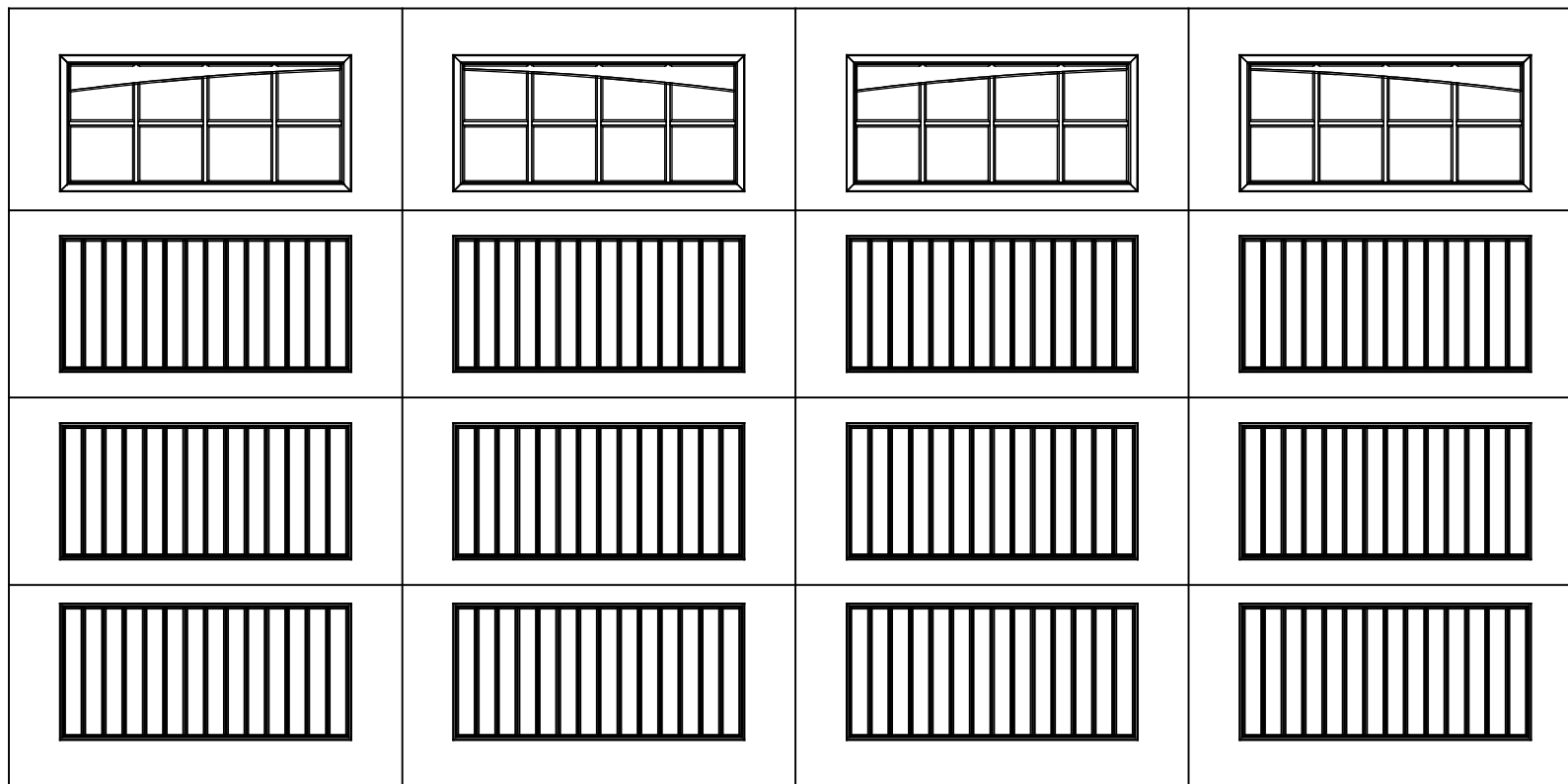
18x9 9800 SONOMA DESIGN 4 SECTION/4 PANEL 32 LITE DOUBLE ARCH TOP SECTION SHOWN CONSISTS OF (2) 25.73" & (2) 27.73" SECTIONS
