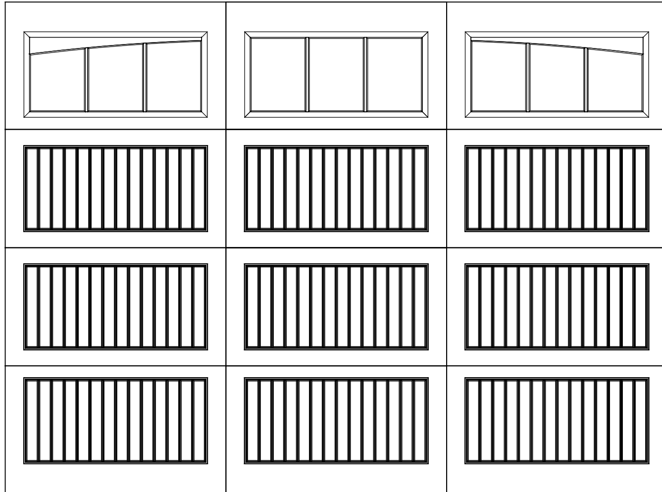
12 X 9 9800 SONOMA DESIGN 4 SECTION/3 PANEL 9 LITE ARCH TOP SECTION SHOWN CONSISTS OF (2) 27.73" & (2) 25.73" SECTIONS
