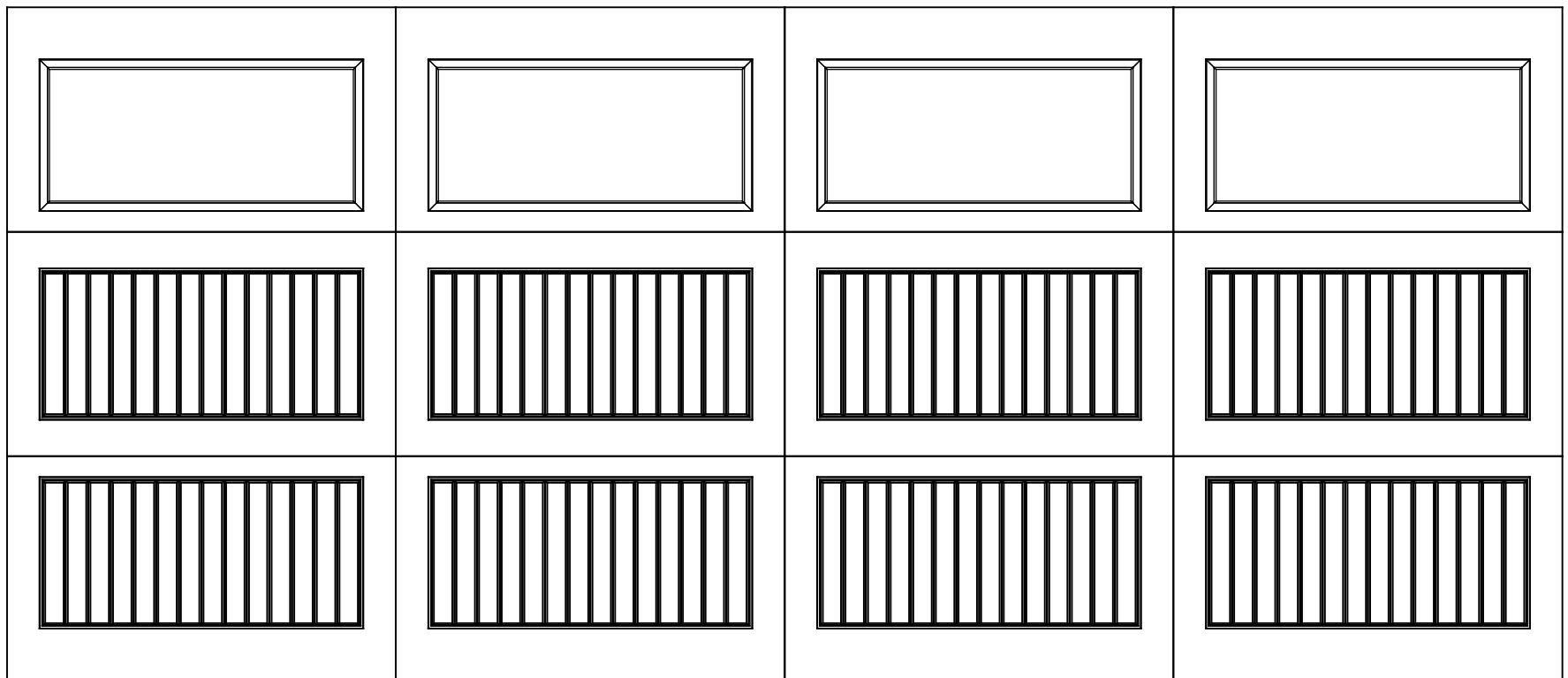
16x7 9800 SONOMA 3 SECTION/4 PANEL PLAIN GLAZED SQUARE TOP SECTION SHOWN CONSISTS OF (3) 27.73" SECTIONS
