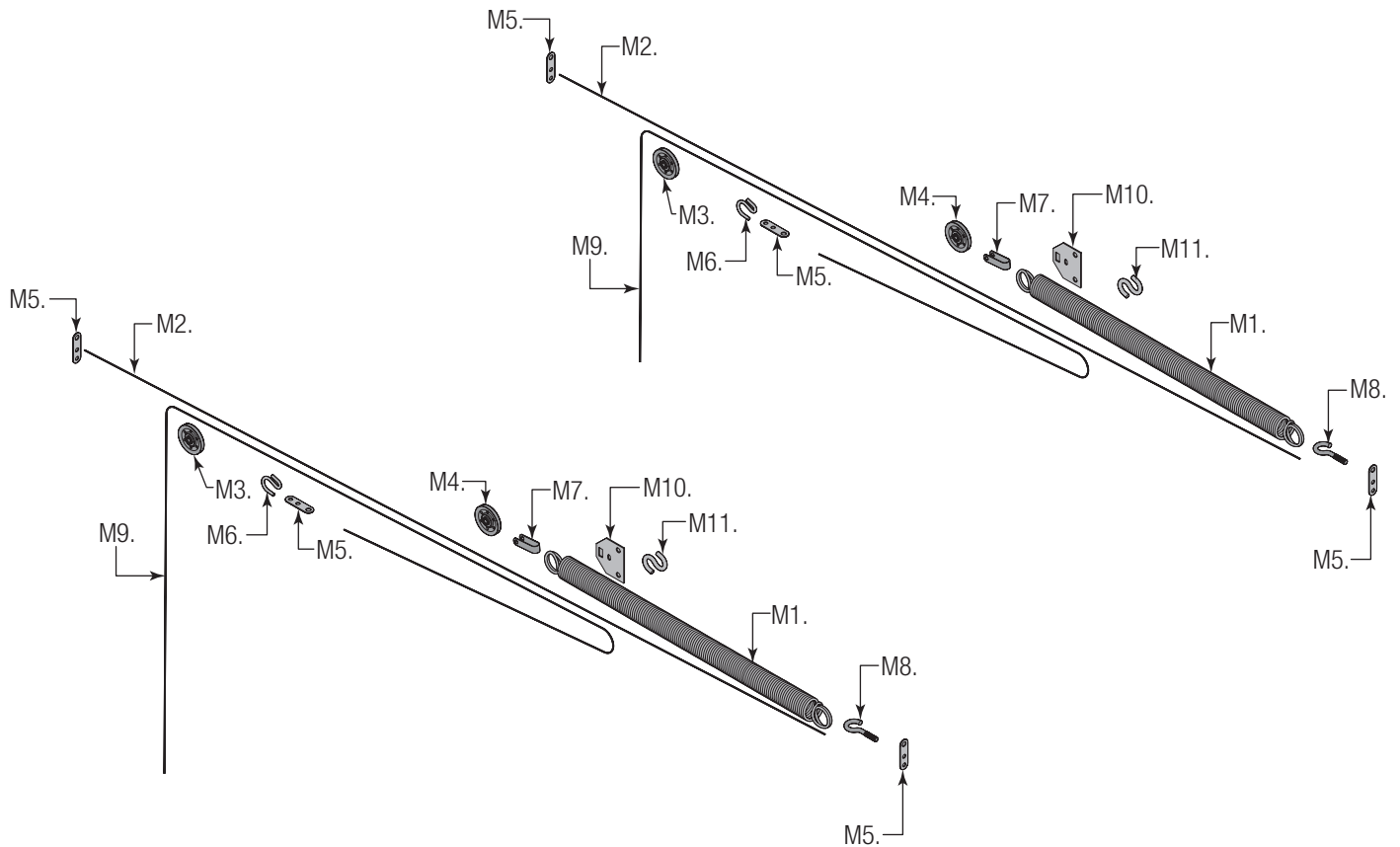
Figure 7 - Counterbalance Components
