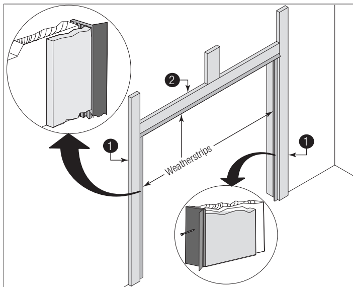
Figure 58, Weatherstrips
