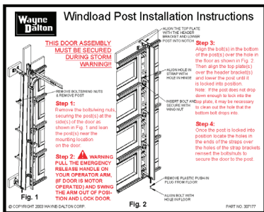
(1) POST INSTALLATION DECAL # 307177
